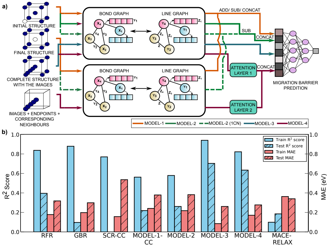
Figure 2: Modified MPT architectures used for FT and train/test scores of different models. (a) The four different modified MPT architectures explored in this work, namely MODEL-1 (orange lines), MODEL-2 (green), MODEL-3 (blue), and MODEL-4 (magenta). Solid (dashed) input/output lines correspond to four (one) convolutions performed on the MPT model. (b) R^2 scores and MAE for all models. The left (blue bars) and right (pink bars) y-axis values represent R^2 scores and MAEs (in eV). Solid and hashed bars denote the train and test scores, respectively.
