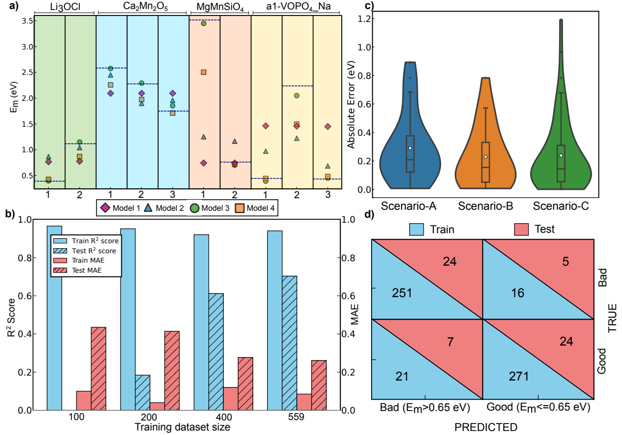
Figure 4: Analysis of model performance. a) Race-track plot illustrating the predictions made by the four different FT models (represented by distinct colored symbols) for different pathways in a given structure. ‘a1’ refers to a specific \text{VOPO}_4 polymorph of space group P4/n . Horizontal lines are the target E_m values for each path. b) Bar chart showing the train and test scores of MODEL-3 with different FT train dataset sizes. c) Violin plot signifying the distribution of absolute errors among the test datapoints under scenarios A (blue), B (orange), and C (green). d) Confusion matrix quantifying the classification performance of MODEL-3 in the train (upper blue triangles) and test (lower pink) datasets.
