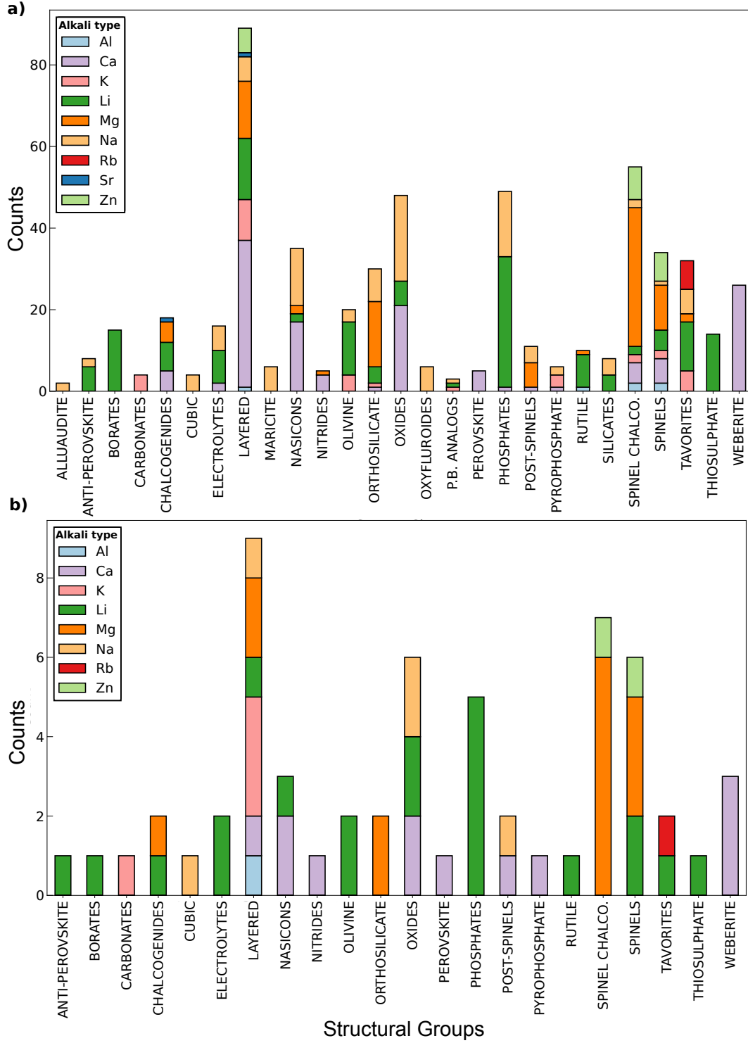
Figure 1: Data distribution of training and test dataset . Distribution of the data in the (a) train and (b) test datasets across different structural groups in the final dataset. The colored stacked bar heights within each bar corresponds to the contribution from different intercalant ions within that structural group.
