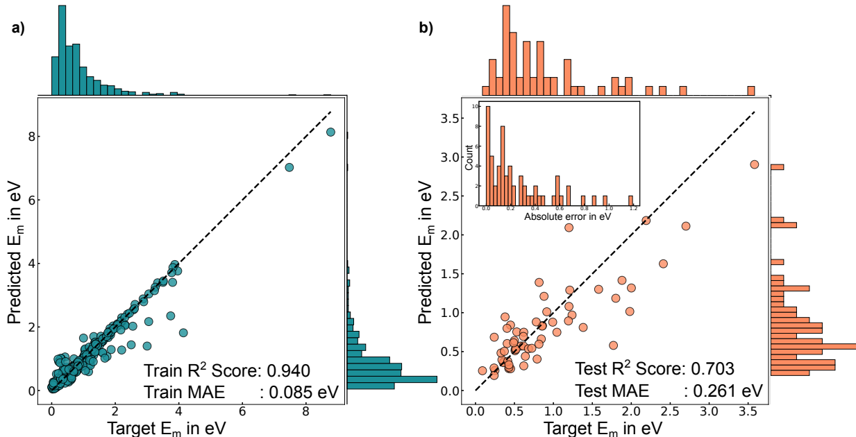
Figure 3: Prediction vs. target E_m . Parity plots for a) training and b) test datasets, respectively. The inset histogram in panel b shows the frequency distribution of the absolute error range in eV. The histograms on the right and top margins illustrate the frequency distribution in the prediction and target E_m in both datasets.
