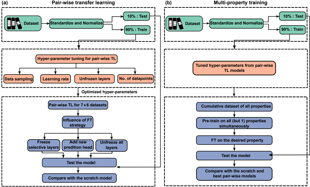
Figure 2: a) Schematic illustrating the workflow (panel a) for pair-wise TL for the seven properties of interest, and (panel b) for MPT.
