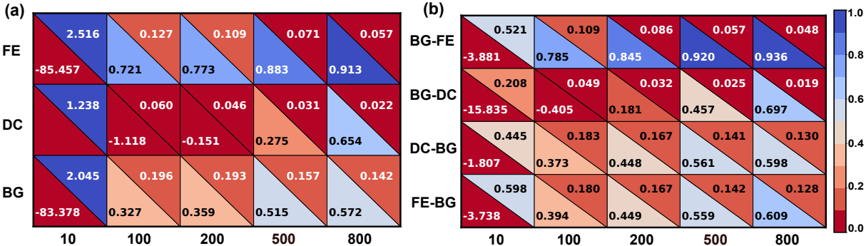
Figure 4: Test R 2 scores (lower triangles) and MAEs (upper triangles) for the models constructed from (panel a) scratch and (panel b) for select PT-FT pairs. The x and y labels in both panels correspond to the dataset size and name or PT-FT pair, respectively.
