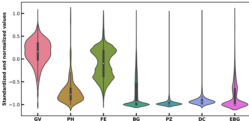
(b) Data distribution for the 7 properties
