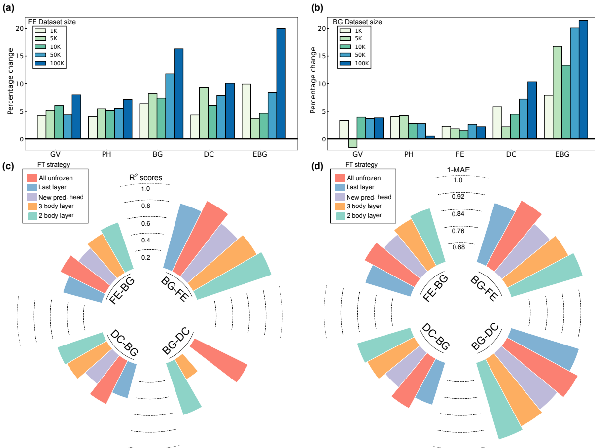
Figure 5: Percentage change in test R^2 scores of PT-FT models with respect to corresponding scratch models, with the PT done on FE (panel a) and BG (panel b). The FT datasets are indicated along the x axis, while the FT dataset size is kept to 800. PT dataset sizes are indicated with different colored bars. Circular bar plots illustrating the performance in terms of R^2 scores (panel c) and 1-MAEs (panel d) for select PT-FT pairs. Different FT strategies are illustrated by the different colored bars. The range of the bars are indicated by the text annotations provided across the concentric circles in both panels.
