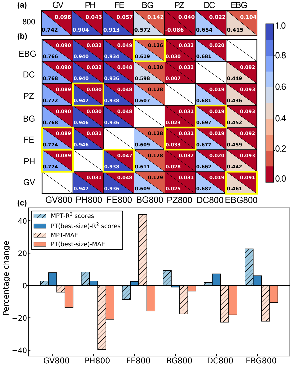
Figure 6: a) R^2 scores (lower triangles) and MAEs (upper triangles) for the models corresponding to the seven datasets constructed from scratch. The x and y labels represent the dataset name and size. b) Performance of pair-wise TL for the 7 \times 6 combinations. The y labels represent the PT datasets, and the x labels display the FT datasets and sizes (i.e., 800 datapoints for all FT). The best performing models are highlighted by yellow boxes. c) Percentage change in R^2 scores (blue bars) and MAEs (orange bars) of the MPT (hashed bars) and PT(best-size)-FT (solid bars) models with respect to scratch.
