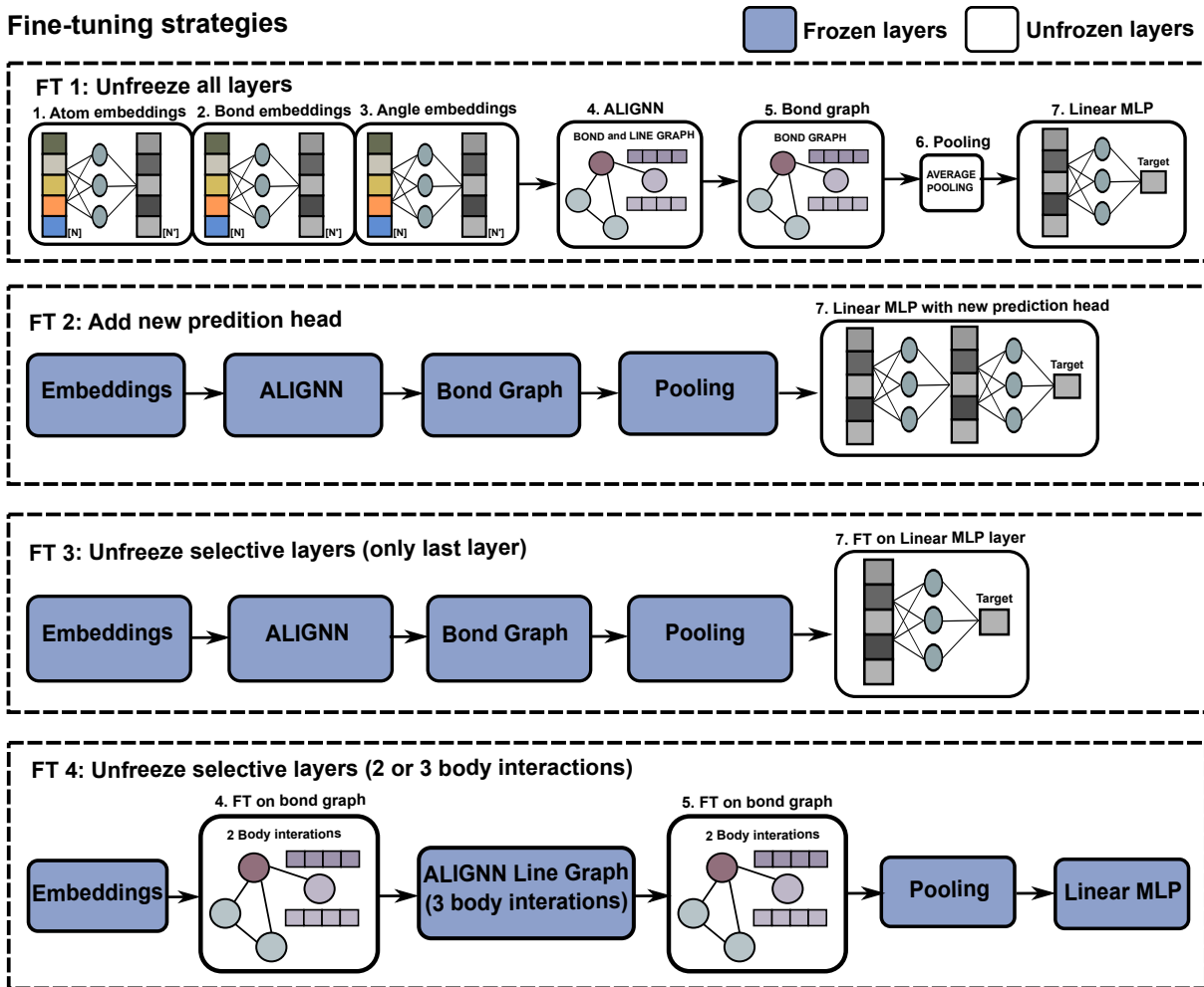
Figure 3: The four FT strategies explored in this work. Blue boxes indicate frozen layers, and unfrozen layers are indicated by black outlined boxes. The contents within each unfrozen layer is indicated in each box, where the notations used within unfrozen layers are identical to Figure 1a.
