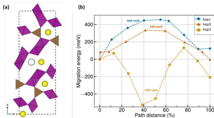
Figure 5. (a) DFT-calculated ground state configuration of Na 0.22 MnO 2 . Brown and purple polyhedra indicate MnO 5 and MnO 6 groups with oxygen atoms occupying the polyhedral vertices. Yellow spheres indicate Na atoms. Black outlined circle indicates a vacant Na site, which is occupied in the case of tt-NMO (see Fig. S3a). (b) DFT-NEB calculated MEPs of Na + migration in Na 0.22 MnO 2 . Blue, red, and orange symbols indicate hops 1, 2, and 3, respectively. Barrier values for each hop is given by the text annotations of the same color. For hop 3, 700 meV is the effective barrier, where the intermediate images have a lower energy than the endpoint configurations.
