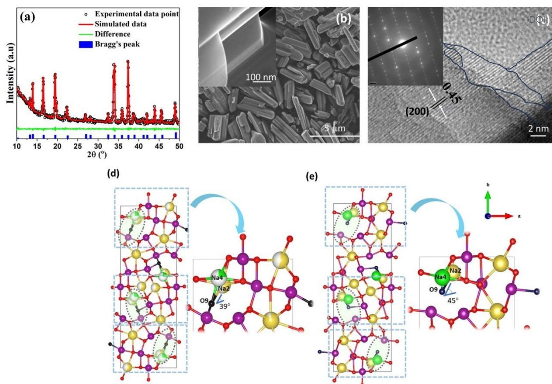
Figure 1: (a) XRD pattern of tt-NMO, (b) Low magnification SEM; inset: High magnification HRTEM, and (c) HRTEM images of tt-NMO; Inset shows the SAED pattern (d) structure of the standard P6mm space group, magnified part of the circled region shows the Na4-O9-Na2 bond angle (e) structure of synthesized tt-NMO; the magnified part of the circled zone clearly indicates the increasing Na4-O9-Na2 bond angle which leads to decrease the bond length and open the channel.
