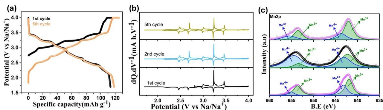
Figure 3: (a) 1 st and 5 th charge-discharge profile of tt-NMO at 0.06C rate (b) dQ \cdot dV^{-1} plot for initial five cycles at 0.06C rate (c) Mn2p XPS spectra of pristine, charged and discharged state.
