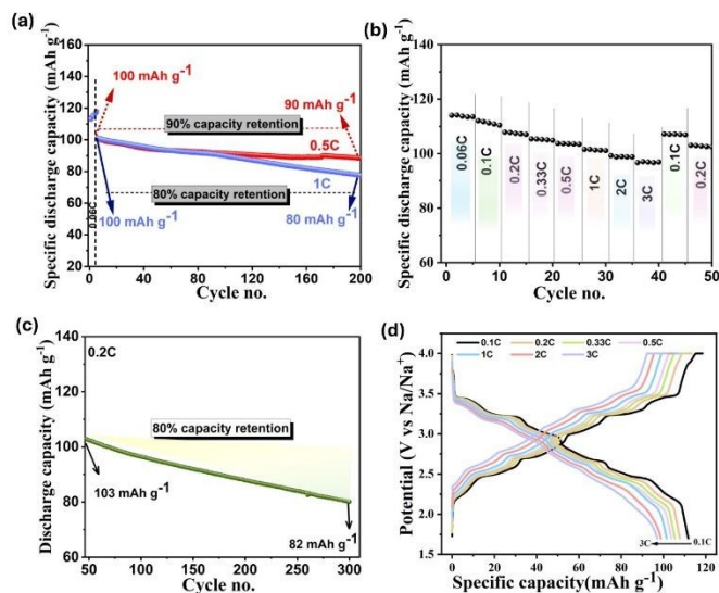
Figure 6 (a) Galvanostatic cycling stability at 0.5C and 1C rate. (b) Rate performance at various current rates. (c) Cycling behavior at 0.2C after rate study. (d) Capacity-voltage profile at different C-rates.
