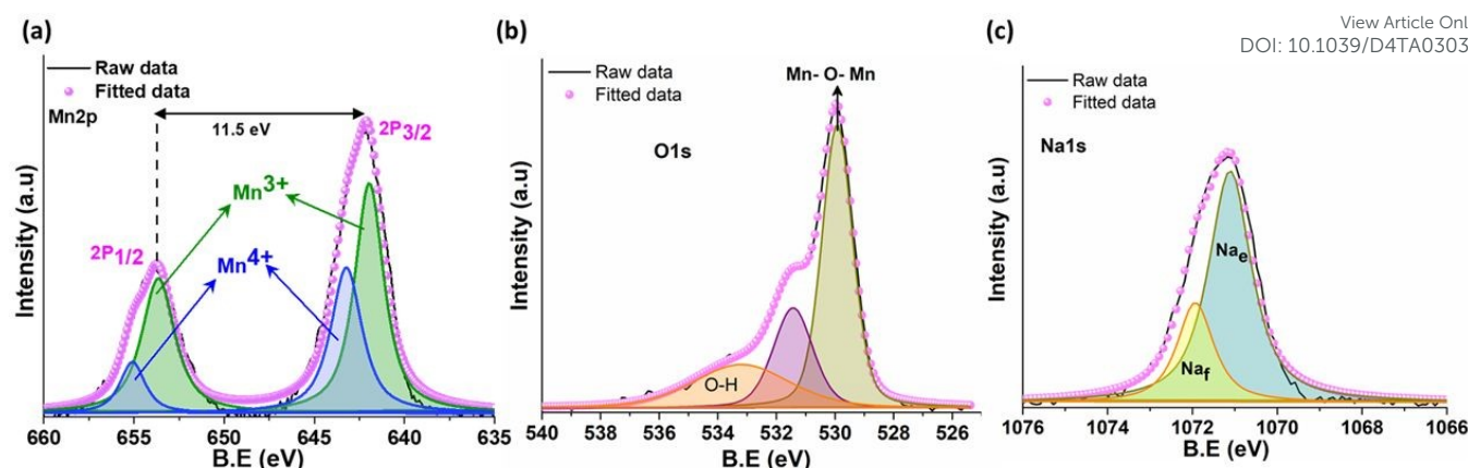
Figure 2: XPS spectra of (a) Mn 2P (b) O1s and (c) Na 1s of tt-NMO
