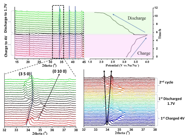
Figure 4: In-situ evolution of XRD pattern recorded at a 12 mA \text{g}^{-1} current rate for the 1 st cycle and a 24 mA \text{g}^{-1} current rate for the 2 nd cycle.
